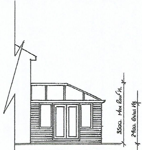
Prop. 4m ELEVATION
